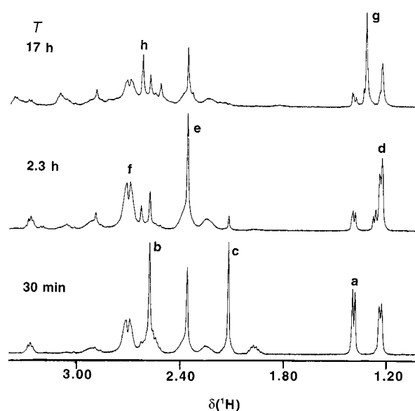
Fig. 4 The 500 MHz ^1\text{H} NMR spectra of [\text{Pt}(\text{en})(\text{Me-Mal-}O,O')] 1 with Gly-Met (5 mM, 1:1 molar ratio) at 310 K and pH 6.66. Peak assignments: a \text{CH}_3 and b \text{CH}_2 (en) for 1 ; c \text{SCH}_3 of free Gly-Met; d \text{CH}_3 , e \text{SCH}_3 and f \text{CH}_2 (en) of [\text{Pt}(\text{en})(\text{Me-Mal-}O)(\text{Gly-Met-S})] 6 ; g \text{CH}_3 of free Me-Mal; h \text{SCH}_3 of [\text{Pt}(\text{en})(\text{Gly-Met-S})_2]^{2+} 7
