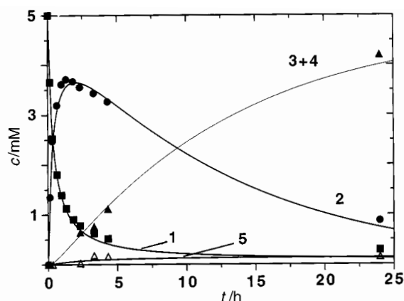
Fig. 3 Kinetic fits for the reaction of [\text{Pt}(\text{en})(\text{Me-Mal-}O,O')] 1 with Ac-Met (5 mM, 1:1 molar ratio) at 310 K and pH 6.56. The curves correspond to the rate constants listed in Table 3
