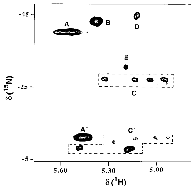
Fig. 2 A two-dimensional [ ^1\text{H} , ^{15}\text{N} ] HSQC NMR spectrum of [\text{Pt}([^{15}\text{N}]\text{en})(\text{Me-Mal-}O,O')] with Ac-Met (5 mM, \text{pH}^* 6.56 , 1:1 molar ratio) recorded at 310 K after 2 h incubation. Peaks assignments: A, \text{NH}_2 ( trans to O) and A', \text{NH}_2 ( trans to S) of [\text{Pt}(\text{en})(\text{Me-Mal-}O)(\text{Ac-Met-S})]^- 2 ; B, \text{NH}_2 ( trans to O) of [\text{Pt}([^{15}\text{N}]\text{en})(\text{Me-Mal-}O,O')] 1 ; C, \text{NH}_2 ( trans to N) and C', \text{NH}_2 ( trans to S) of [\text{Pt}(\text{en})(\text{Ac-MetH}_{-1}\text{-S,N})] 3 . Peaks D and E for impurities {hydroxyl bridged [\text{Pt}(\text{en})]^{2+} complexes and [\text{Pt}([^{15}\text{N}]\text{en})\text{Cl}_2] } contained in the stock solution of complex 1
